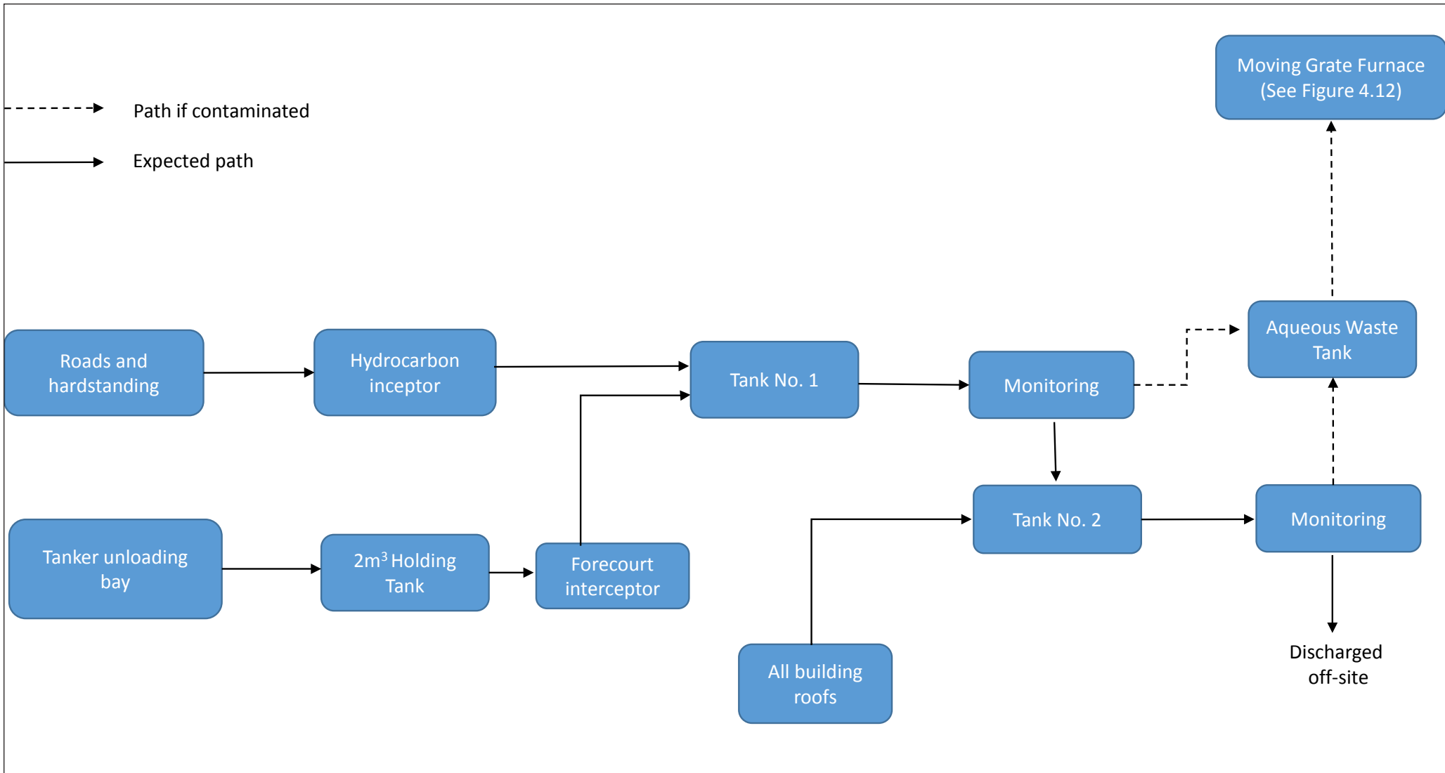
Figure 4.18 Schematic of Stormwater Management System
