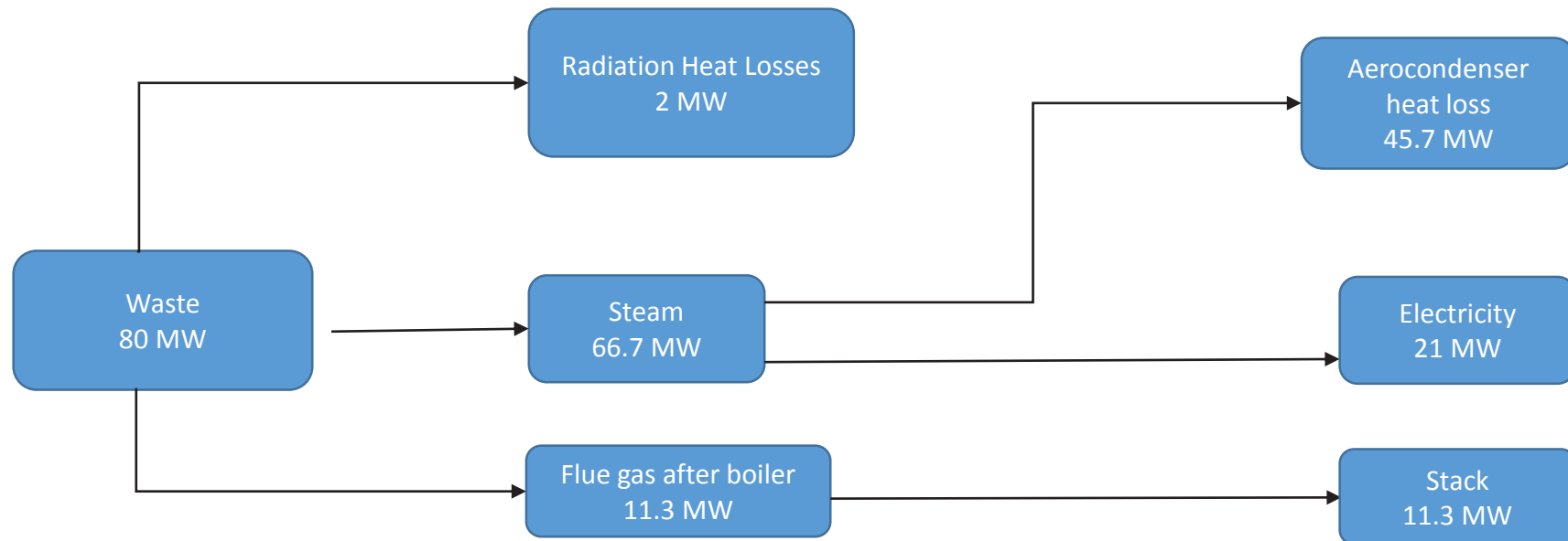
Figure 4.16 Schematic of Heat Balance
