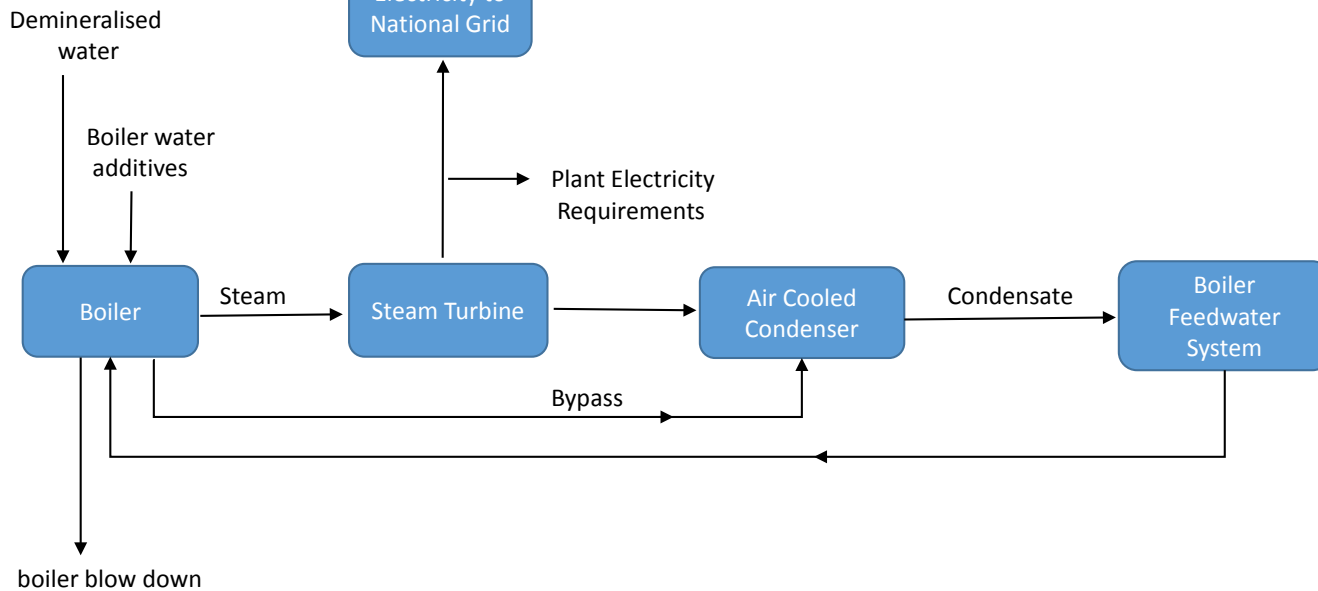
Figure 4.14 Schematic of Steam Turbine
