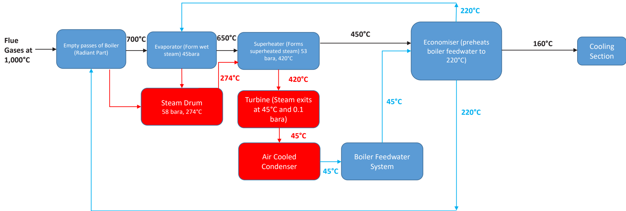
Figure 4.13 Schematic of Boiler
