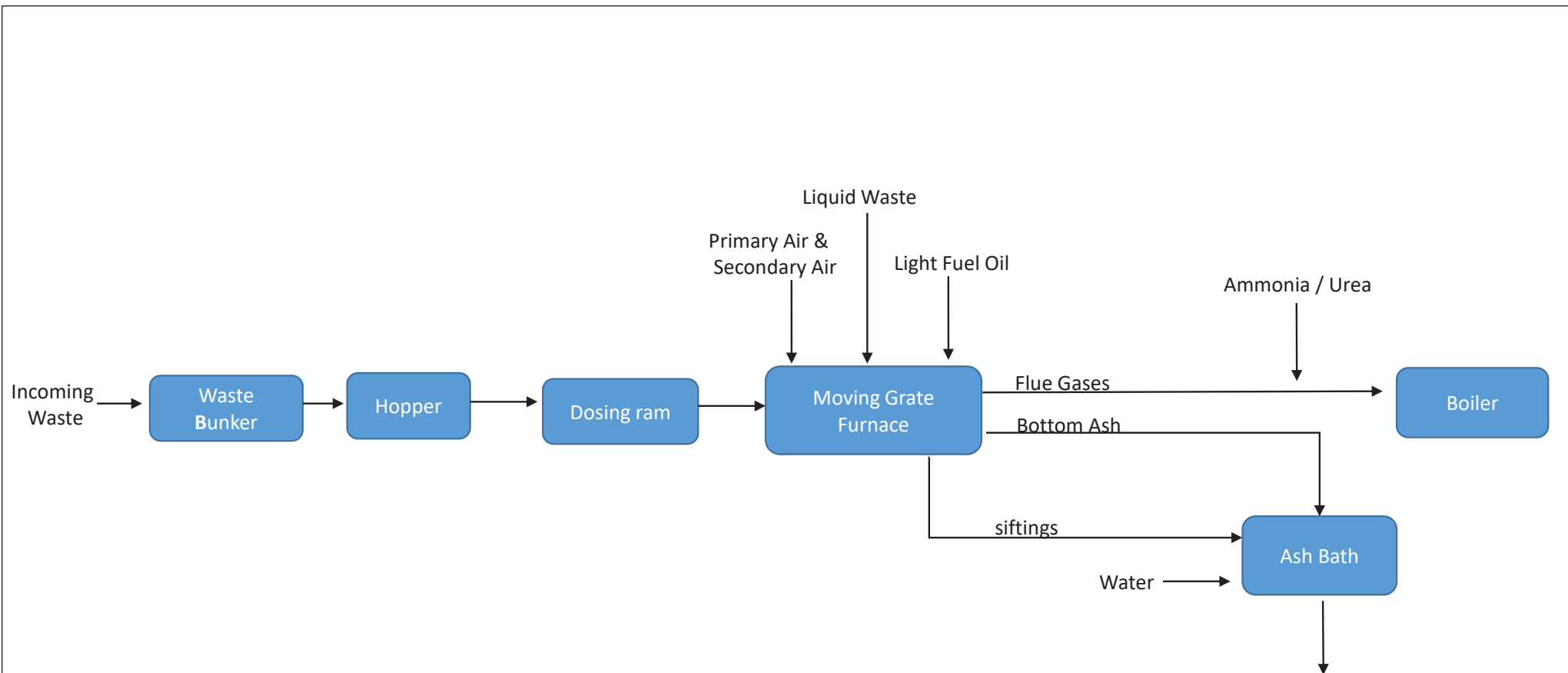
Figure 4.12 Schematic of Moving Grate Furnace
